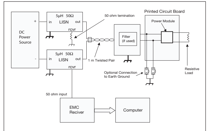
Test set-up.
